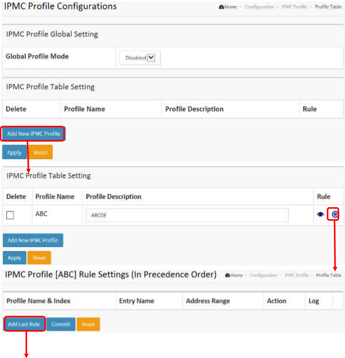
Figure 2-9.1: The IPMC Profile Configuration
